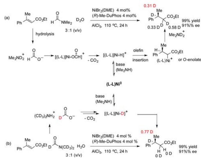
Scheme 3. Deuterium-Labeling Experiments
